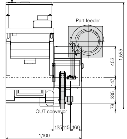
IN part feeder / OUT conveyor
