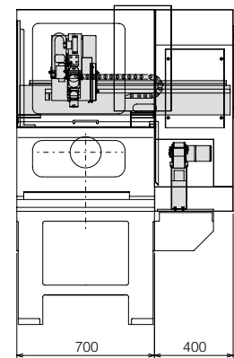
IN/OUT workpiece stocker
