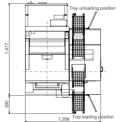
IN/OUT workpiece stocker
